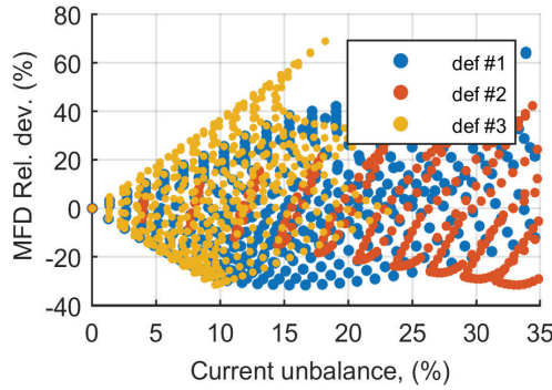
Figure 7: Relation between current unbalance and deviation of the magnetic flux density for Case 2, and Subcase c, calculated at h=1\text{m} . I_1=100\text{A} , while I_2 and I_3 are in a range from 60A to 140A
