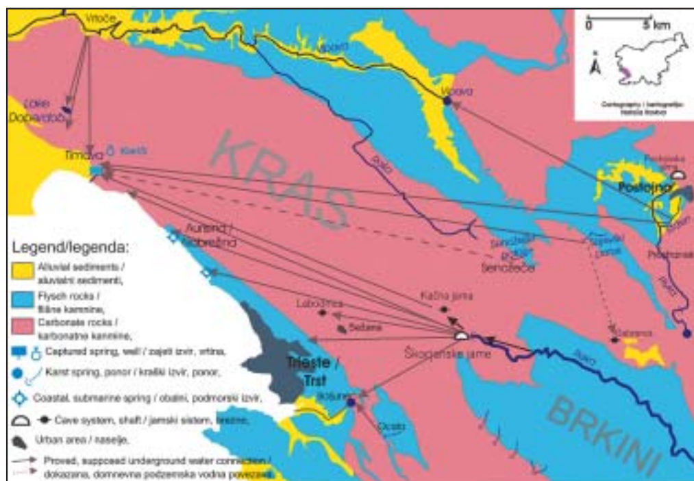
Figure 1: Simplified geological map of the Kras plateau with proved and supposed groundwater connections (Civita s sodelavci 1995; Buser et al. 1963; Buser 1964; Gemiti 1984; Pleničar et al. 1965; Timeus 1928).
