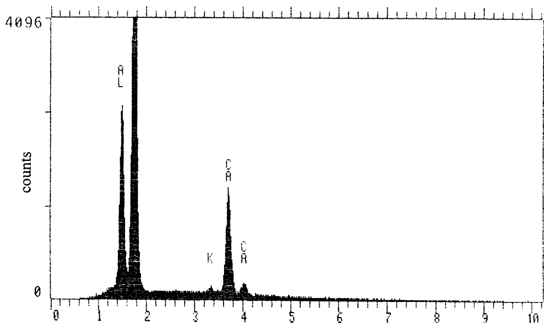
Figure 3. Energy dispersive x-ray spectrum (EDX) of laumontite
