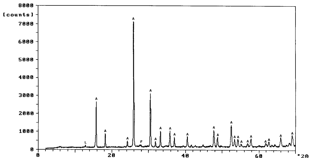
Figure 2. X-ray diffraction pattern of analcime, separated from an analcime-rich rock
