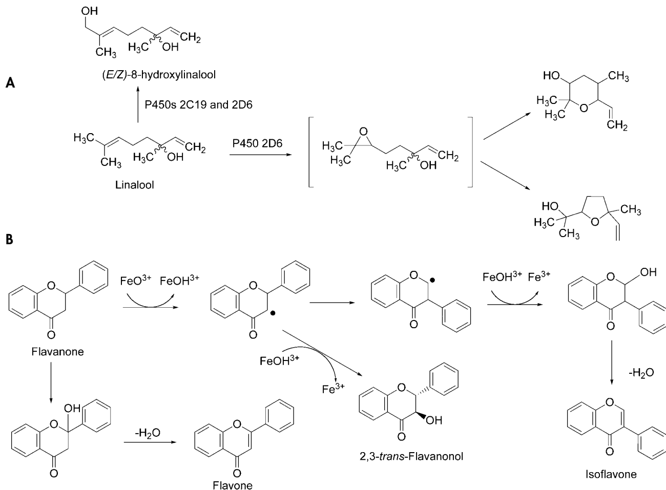
Fig. 7. Rearrangement reactions initiated by P450s. A , Epoxidation of linalool by P450 2D6 followed by spontaneous rearrangement to give cyclic ethers. B , Rearrangement of flavanone to isoflavone following hydrogen atom abstraction by P450.
