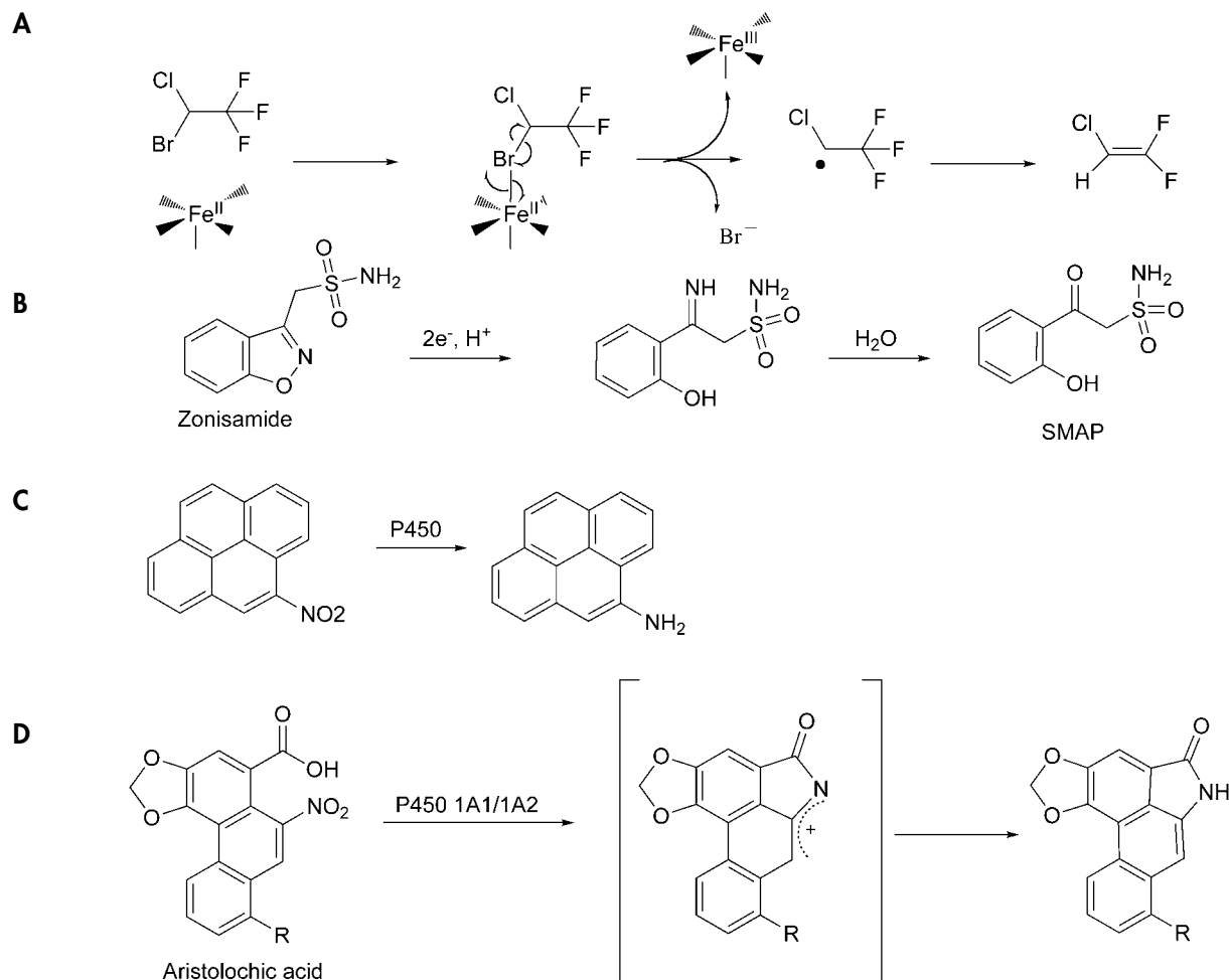
Fig. 6. Examples of reduction reactions catalyzed by P450s. A , Reductive dehalogenation of haloethane via "Type II" binding to reduced heme iron. B , Reductive ring cleavage of the anticonvulsant drug zonisamide by P450. C , Reduction of 4-nitropyrene to 4-aminopyrene. D , Reductive cyclization of two aristolochic acid components via the formation of a nitrenium intermediate.
