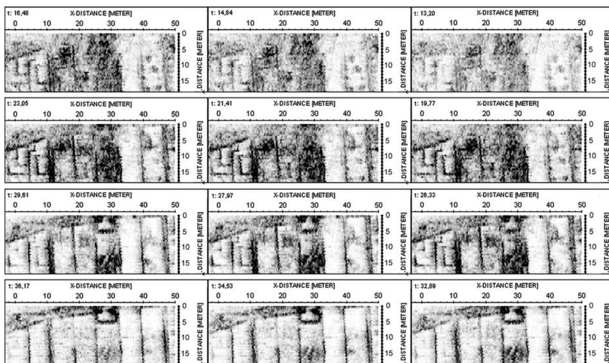
Fig. 18: Structures 3, 4 and 5, the northern defence wall and tower and the paved road (see Fig. 36), GPR area G3 (Fig. 3C), measured surface of 53 x 20 m: time slices. The single and double walls of the storehouse rooms 3, 4 and 5 are discernible, as well as the numerous walls that divide the interiors of the rooms. Some of these small rooms are paved. That the northern wall seems to be double is consequent to the paved platform on the outside of the defence wall and the wall that runs almost parallel with it. The 1 m wide walls of the northern tower are discerned at the approximate depth of the paved road, which runs from the northern gateway to the interior of the settlement. The tower is clearly distinguished only under the paved road; presumably it is not preserved higher up. Approximately in the centre of the tower is a narrowing with a passage into the interior of the settlement. The northern tower has the deepest foundations (reaching to a depth of 1.6 m) within the geophysically explored part of the settlement.
