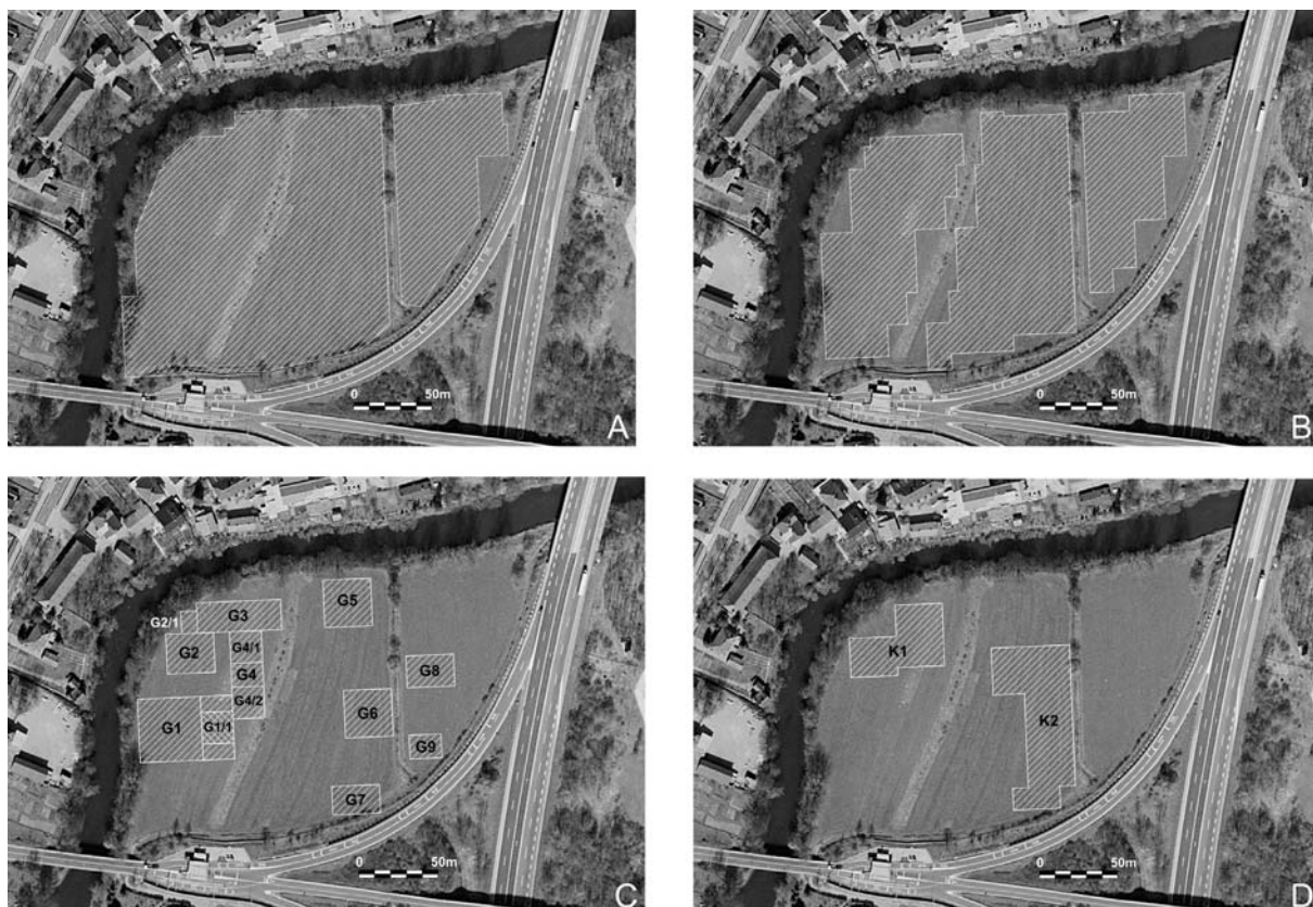
Fig. 3A-D: Areas investigated using the geoelectric resistivity method (A), the magnetic method (B), the Ground Penetrating Radar method (C: G1-G9) and the electrical conductivity method (D: K1-K2) (Source: © Surveying and Mapping Authority of the Republic of Slovenia, DOF at a scale of 1 : 5000).
