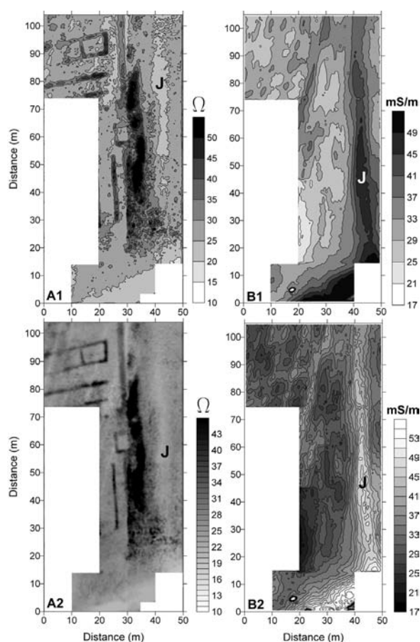
Fig. 15: The course of the defence ditch is traceable in the resistivity results (A1 and A2: J), however it is more discernible on the electrical conductivity results (B1 and B2: J).
