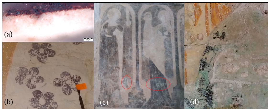
6. Colour darkening due to pigment degradation, observed on the sample microphotograph (a) and in situ (b, c, d) in the following locations: (a, b) Pb pigment (?), St Peter's church in Ribičje, (c) Pb and/or Cu pigments, St James's church in Ormož (central nave), and (d) malachite, St Nicholas's church in Žužemberk (St. Erasmus) ((a) © IPCHS, RC, Scientific department; (b-d) photos: Anabelle Križnar).
