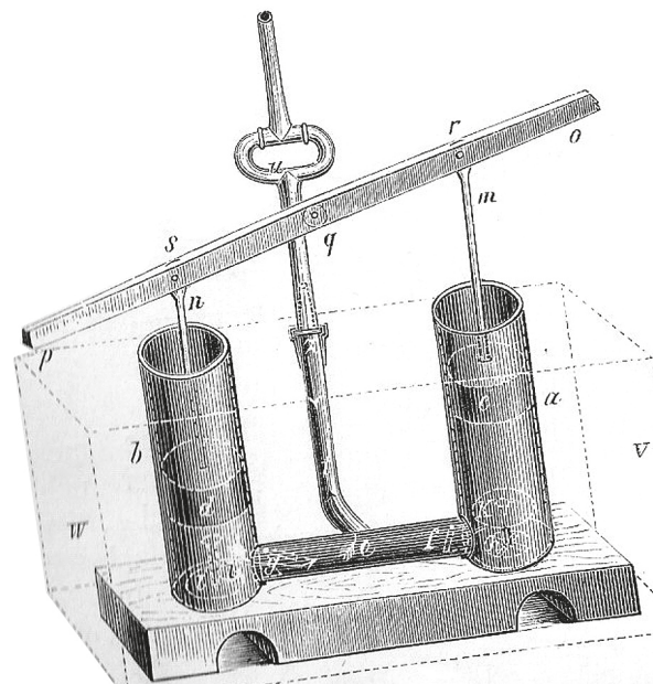
Heronova brizgalna
