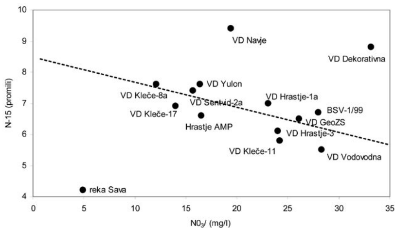
Figure 8. Average \delta^{15}\text{N} isotope composition in the nitrates in the groundwater of Ljubljansko polje versus nitrate concentration.
