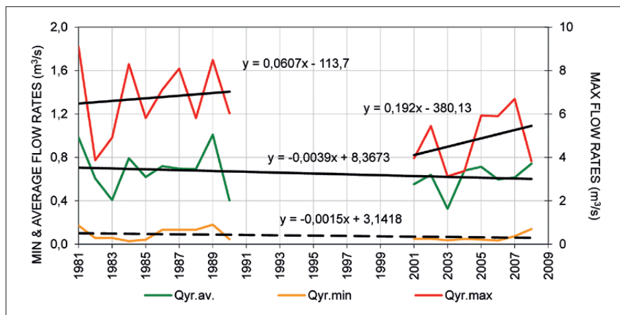
Fig. 6: Time series of minimum, average and maximum annual flow rates at the gauging station Plitvica Bridge for the period 1981–2008 (Meaški 2011).
