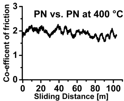
Fig. 13. The variation of COF as a function of sliding distance at 400^\circ\text{C} for the PN coated ring - PN coated pin Pair
