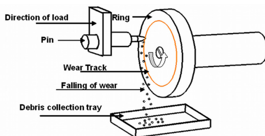
Fig. 3. Schematic diagram of loading configuration of VPOD
