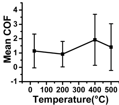
Fig. 9. The Error bar for the mean COF at 25, 200, 400 and 500 °C
