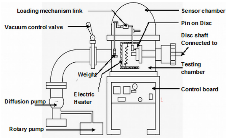
Fig. 1. Schematic view of the vacuum based high temperature Pin-On-Disc machine
