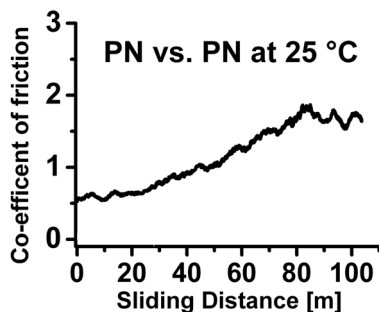
Fig. 7. The variation of COF as a function of sliding distance at 25\text{ }^{\circ}\text{C} for the PN coated ring - PN coated pin Pair
