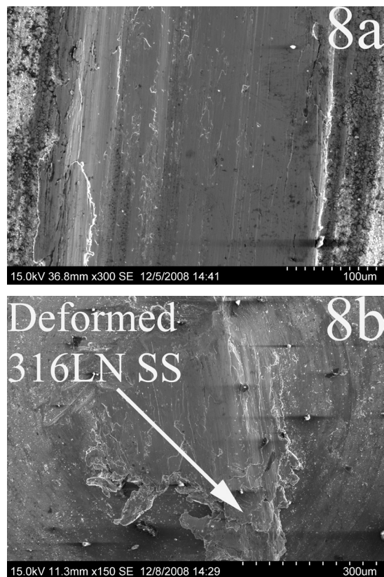
Fig. 8. SEM micrograph taken after tribological test for PN coated ring-PN coated pin Pair at 25\text{ }^{\circ}\text{C} ; a) wear track generated on PN ring; b) surface of the PN coated pin
