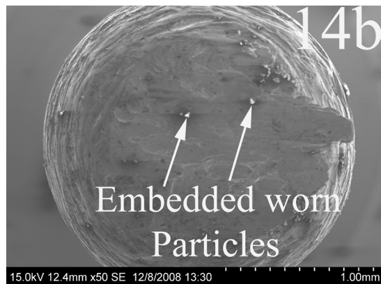
Fig. 14. SEM micrograph taken after tribological test at 400^\circ\text{C} for PN coated ring - PN coated pin Pair; a) Wear track generated on PN ring; b) surface of the PN coated pin
