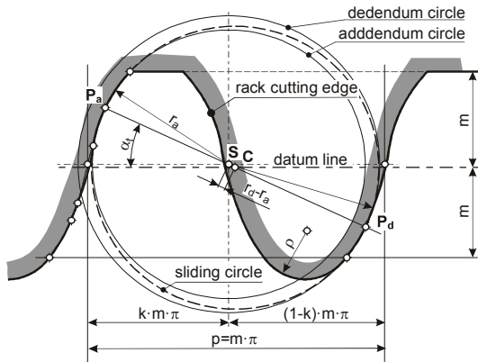
Fig. 4. UPT rack profile
