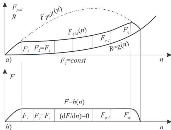
Fig. 6. Function F_{\theta_{\Delta T}}(n) of acceleration with constant difference F_q = \text{const} in relation to resistance a) R = g(n) of the road and b) force F = h(n) which accelerate vehicle
