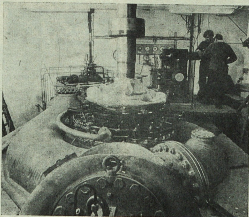
Turbina v HE Mangapapi pred pogonom
