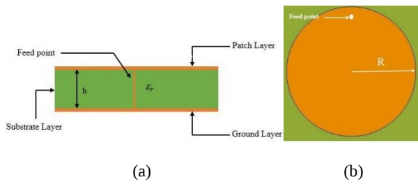
Figure 1 . Conventional CMPA produced by FEKO, (a): Side view (b): Top view
