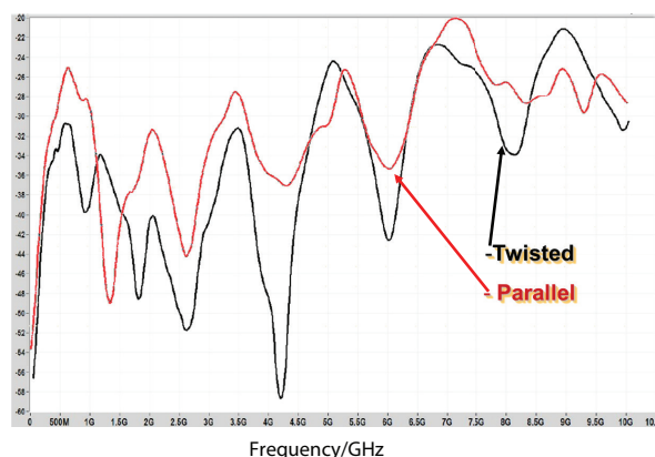
Figure 3: S21 data-Crosstalk for ST with 1 mm-distance for parallel and twisted pairs of 135 \mu\text{m} diameter wires.
