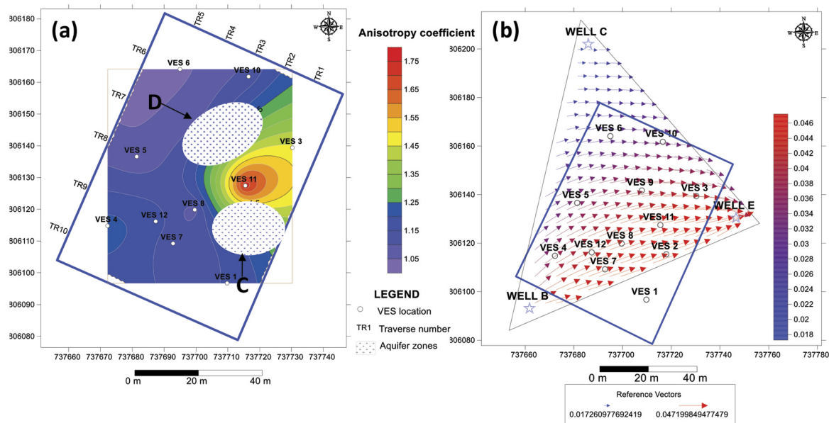
Figure 7: (a) Coefficient of anisotropy map. (b) Hydraulic gradient vector plot of groundwater flow magnitude and direction.
