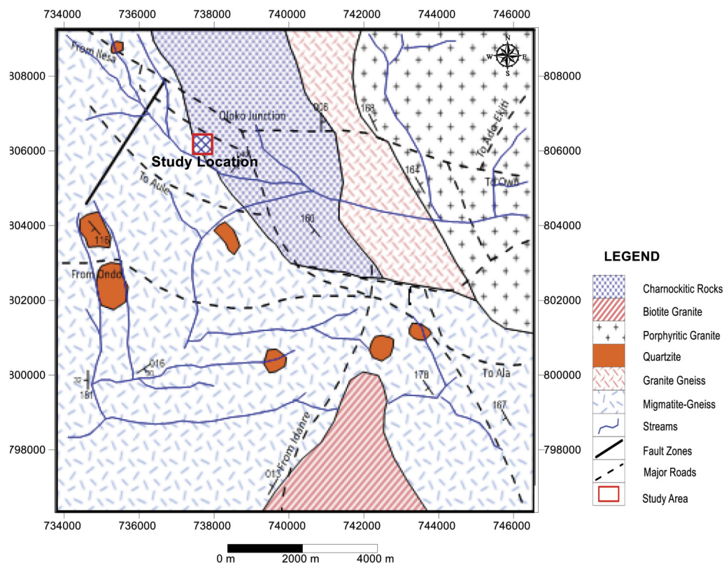
Figure 2: The study area identified on a simplified geological map of Akure [27].
