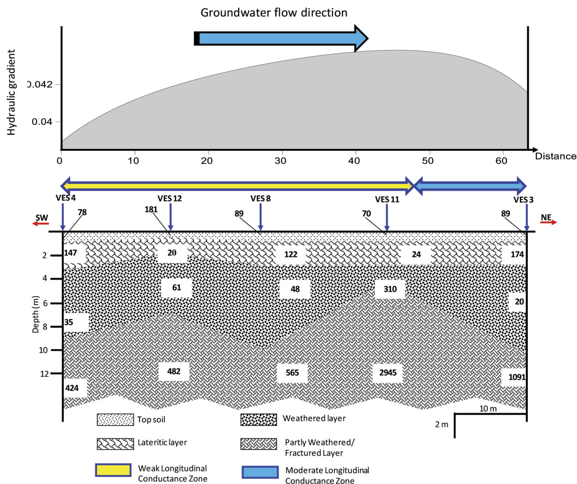
Figure 8: Profile of hydraulic gradient and geoelectric section along an arbitrary profile, integrated with the longitudinal unit conductance.
