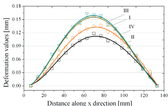
Fig. 5. Specimen deformation of 0.75 mm thickness plate
