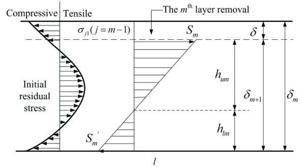
Fig. 1. Initial residual stress and additional stresses after the removal of materials
