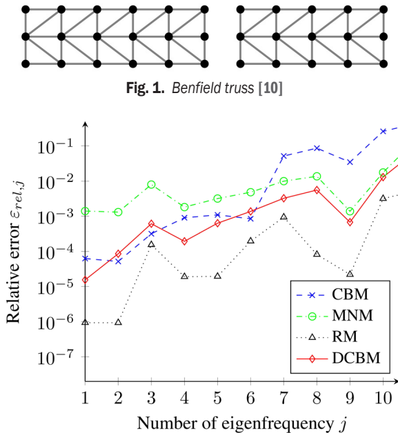
Fig. 2. Relative error of eigenfrequency using 5 normal modes per substructure for the approximation of the lowest eigenfrequencies of the Benfield truss
