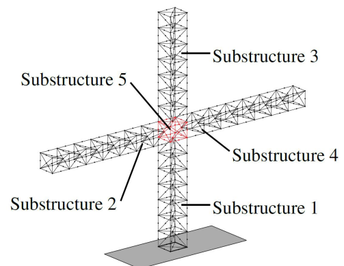
Fig. 7. Frame made of steel beams divided into 5 substructures [6]
