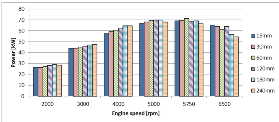
Figure 4: Numerical results of engine-rated power with different trumpet lengths
