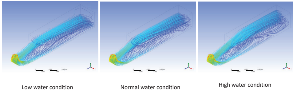
Figure 7: Velocity streamlines
