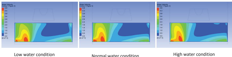
Figure 8: Velocity contours
