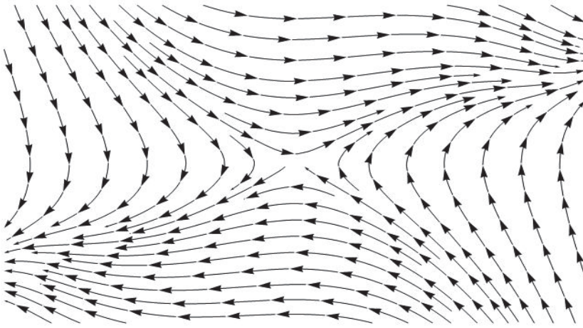
Figure 9: Phase portrait of a saddle for (1.5); a_2 = a_4 = 0 , a_3 = 1 , c_1 = -1 , c_3 = c_5 = 0 , c_7 = 1
