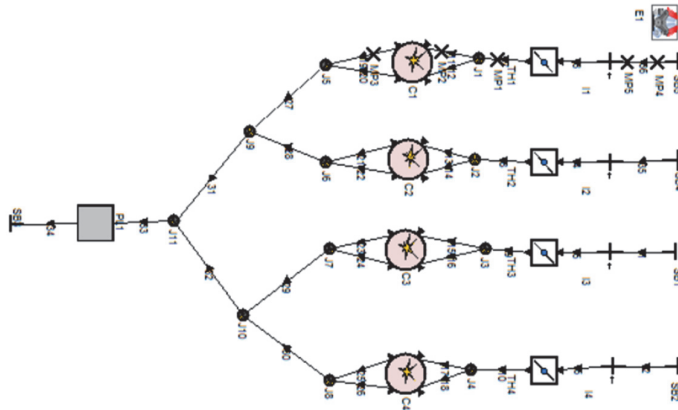
Figure 1: Engine model in BOOST
