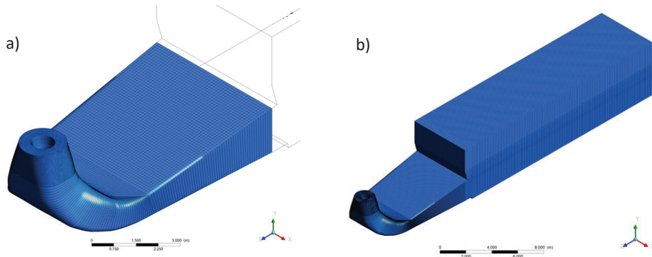
Figure 2: Numerical mesh a) draft tube and b) draft tube with prolongation
