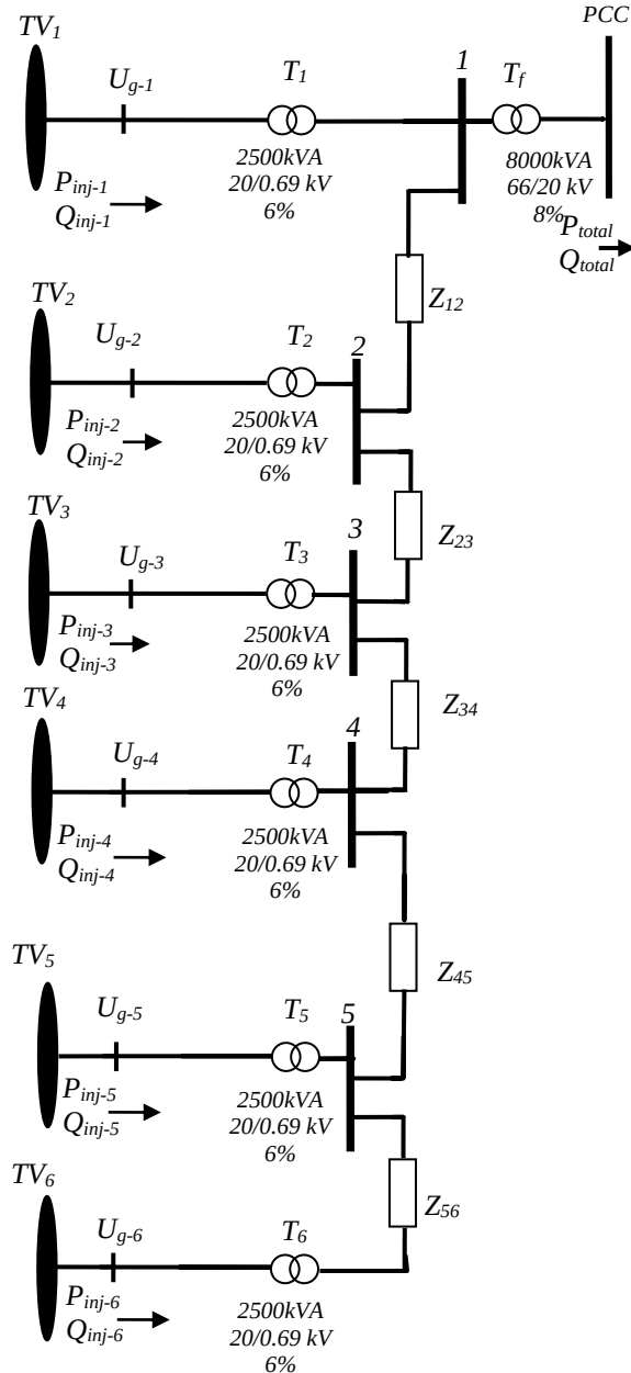
Figure1. Layout of the studied wind farm.
