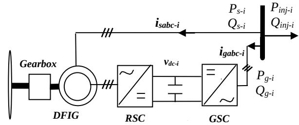
Figure2. Scheme of the i^{th} WECS of the studied wind farm.
