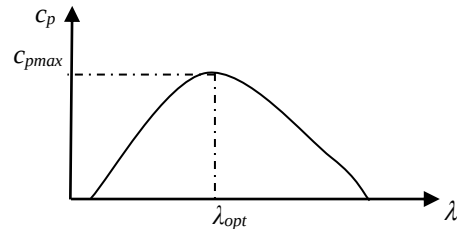
Figure 3. Power coefficient versus the tip-speed ratio.
