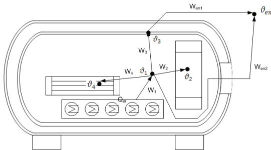
Fig. 2. Scheme for the heating process modelling
