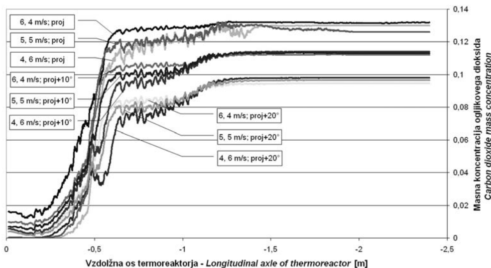
Sl. 14. Vpliv smeri in hitrosti dovajanja zraka na povprečen nastanek \text{CO}_2 Fig. 14. Air-intake direction and velocity influence on average \text{CO}_2 formation
