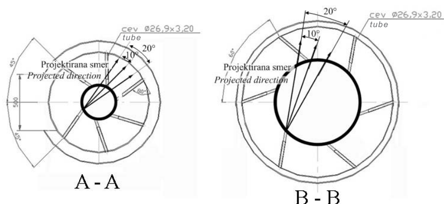
Sl. 12. Projektirane in spremenjene smeri dovoda sekundarnega in terciarnega zraka Fig. 12. Projected and altered directions of secondary and tertiary air inlets
