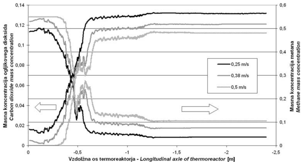
Sl. 11. Vpliv količine plinov iz primarne komore na porabo metana in nastanek \text{CO}_2 Fig. 11. Primary chamber gas amount influencing fuel consumption and \text{CO}_2 production
