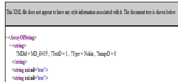
Figure 22: MD_check result.
