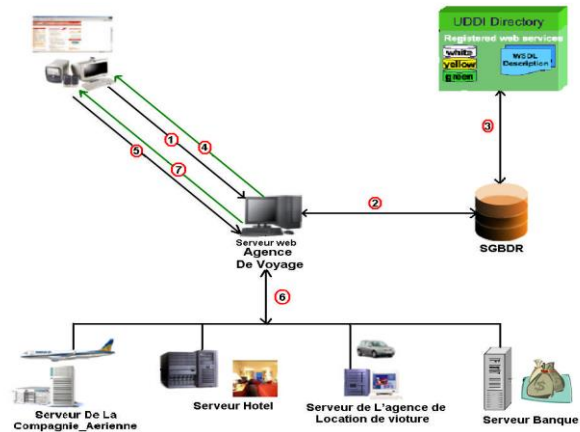
Figure 17: Global architecture of the application.
