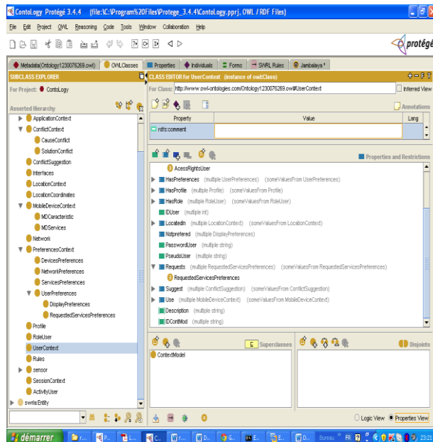
Figure 5: Contology classe and properties creation.
