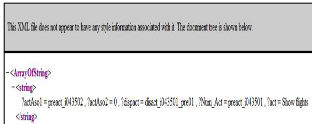
Figure 21: Service_check result.
