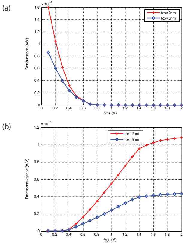
Figure 9: Effect of oxide thickness on the (a) conductance at V_{gs} = 1 V and (b) trans-conductance at V_{ds} = 1 V.
