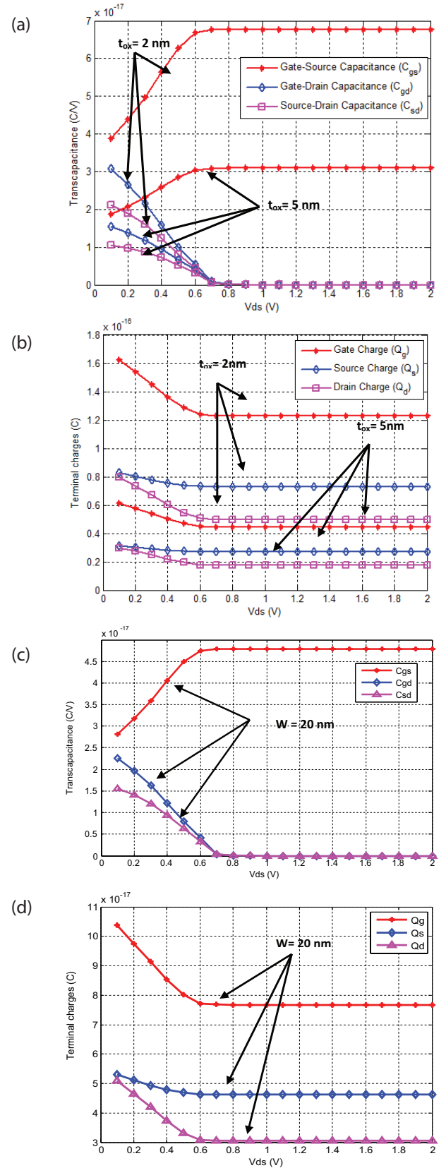
Figure 10: (a) Trans-capacitance, (b) terminal charges for W = 30 nm and L = 90 nm, (c) Trans-capacitance, and (d) terminal charges for W = 20 nm, t_{ox} = 2 nm and L = 90 nm, at V_{gs} = 1 V.
