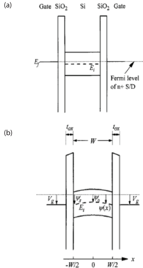
Figure 3: The band model of the symmetric DG MOSFET a) V_{gs} = 0 V b) V_{gs} = V_{th} [9].
