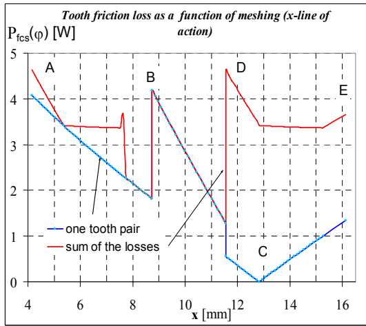
Fig. 3. The apparent power loss generated by the tooth friction between sun gear and planet gear of a planetary gear K+K (Input power: P_{in}=500 [W], tooth numbers: z_2=31 , z_3=30 , center distance: a_w=76,25 [mm] profile shift factor of sun gear x_2=0,5 , profile shift factor of planet gear x_3=-0,5 , gear ratio: i=15,7541 , input speed: n_{in}=1440 [1/min], point C is the pitch point)
