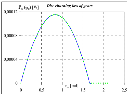
Fig. 13. Disc churning loss of a planet gear
