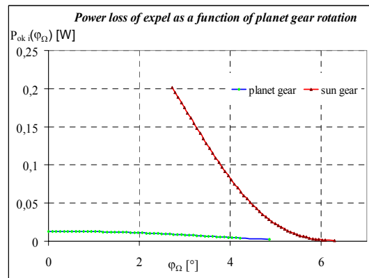
Fig. 8. Power losses generated by oil expel in a planetary gear K+K (Input power: P_{in}=500 [W], tooth numbers: z_2=31 , z_3=30 , z_2'=30 , z_3'=31 , center distance: a_w=76,25 [mm], gear ratio: i=15,7541 , input speed: n_{in}=1440 [1/min], dip lubrication)
