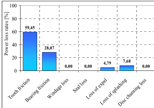
Fig. 16. The constituents of the total power losses for a planetary gear K+K (Input power: P_{in}=500 [W], tooth numbers: z_2=31 , z_3=30 , z_2'=30 , z_3'=31 , center distance: a_w=76,25 [mm], gear ratio: i=15,7541 , dip lubrication)
