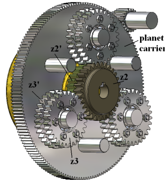
Fig. 15. The investigated planetary gear K+K
