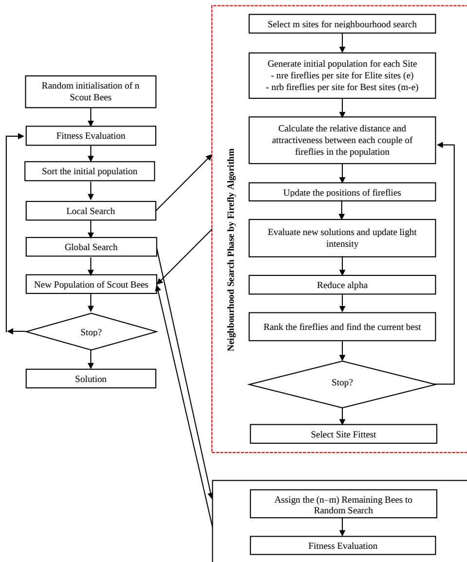
Figure 6: Flow chart of Hybrid Bee Firefly Algorithm (HBAFA).
