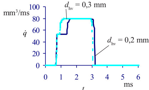
Sl. 7. Vpliv premera izvrtine hidravličnega ventila ( h_{nl} = 0,07 mm, 3/2 sv) Fig. 7. The influence of the nozzle of the hydraulic valve diameters ( h_{nl} = 0,07 mm, 3/2 sv)
