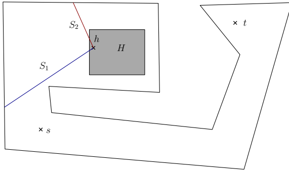
Figure 7: The removal of the segments S_1 and S_2 splits P into two connected components. s and t lie in the same connected component.
