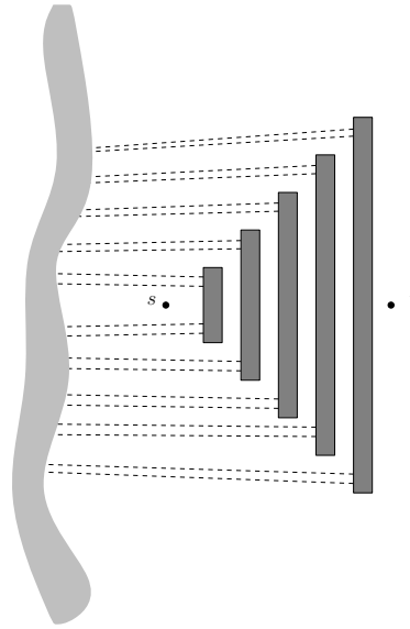
Figure 6: Far away on the right side portions of visibility regions hit the rectangles corresponding to edges.
