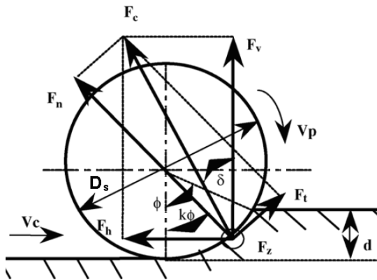
Fig. 14. The kinematics of basic machining process [6]
