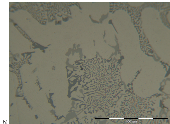
Fig. 4. Microstructure of the laser surface modified layer of AlSi12CuNiMg alloy; a) remelted zone, b) transition zone
