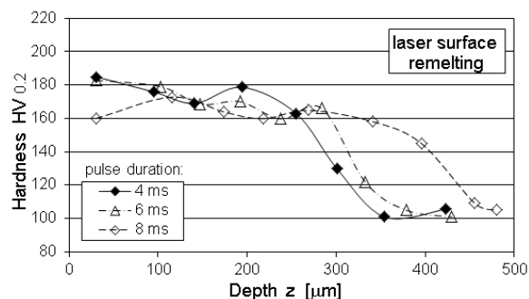
Fig. 5. Micro-hardness measurements through the laser modified surface layer
