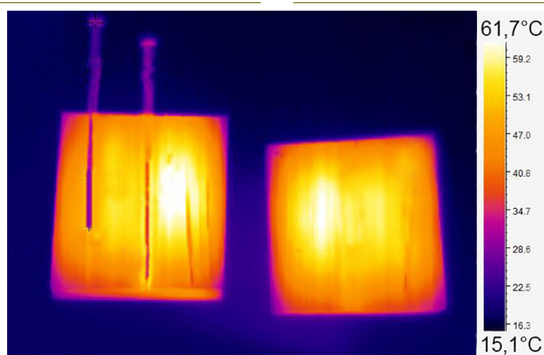
Fig. 9: Heating of metal in the wood
