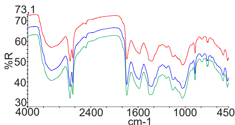
Fig. 8: FT-IR spectra of oil paint that was dried for 6 months (above) and then exposed to 60°C (middle) or 80°C (below)
