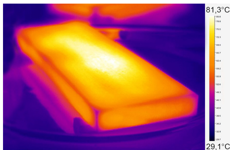
Fig. 1: Heating the surface of the sample with sandarac lacquer
