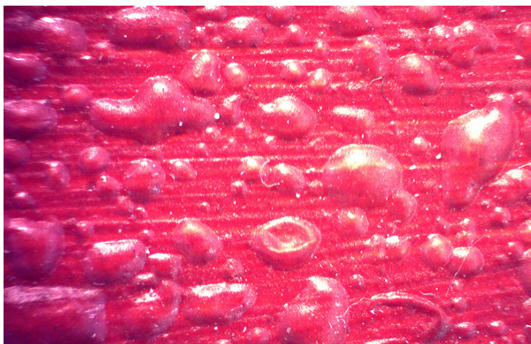
Fig. 2: Blistering of incompletely cured oil paints when exposed to 79.5° C for 10 minutes. 10 times magnification
