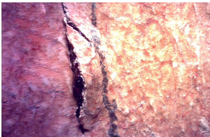
Fig. 6: An oil marbling crack formed due to the melting and penetration of wood resins to the surface at a temperature of 78.5°C. 10 times magnification.
