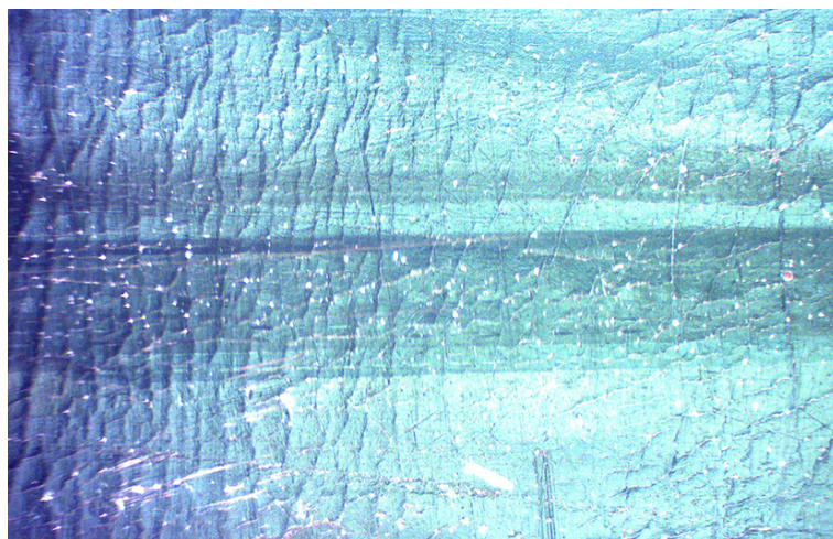
Fig. 5: The resulting cracks on the sample with polished silvering on exposure to 79° C and 10 minutes. 10 times magnification.
