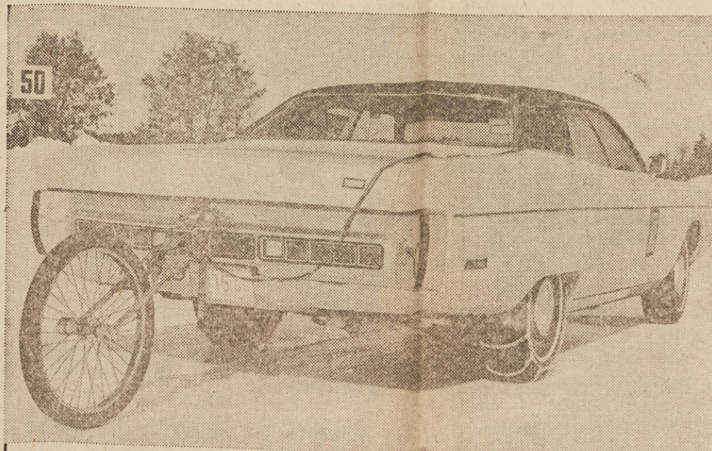
CHAINED UP AND READY TO GO—This test car is "chained up" and ready for a run at the National Safety Council's winter test site in Stevens Point, Wisconsin. The trailing "fifth wheel" is used to make precise measurements of both speed and distance.
