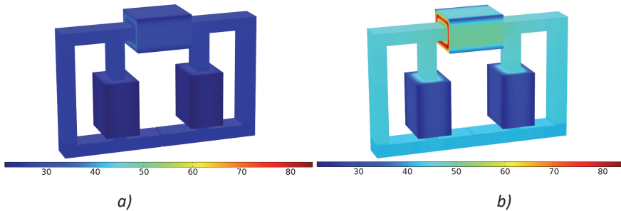
Figure 9: Thermal field distribution ( ^{\circ}\text{C} ) in HEMSMM at operating time 2h and supply voltages: a) 6V; b) 12V
