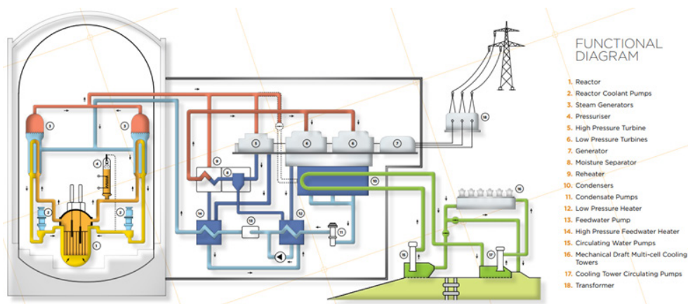
Figure 1: Functional diagram of NPP Krško; source: www.nek.si
