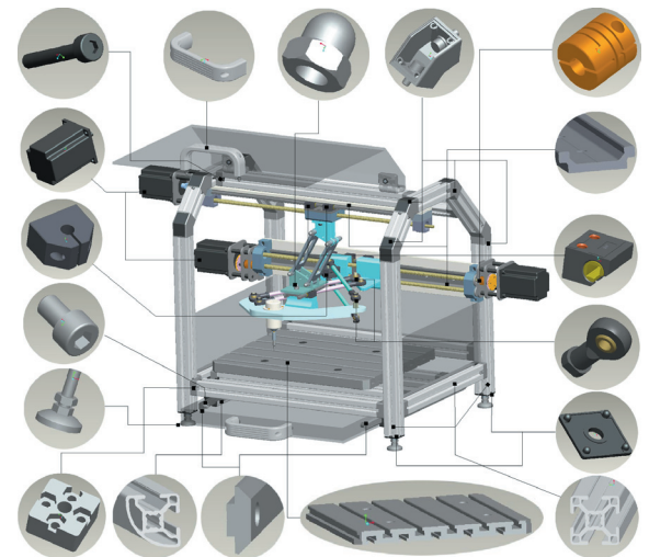
Fig. 11. Mini-laboratory and desktop 3-axis PKMM - pn101_st V2.5
