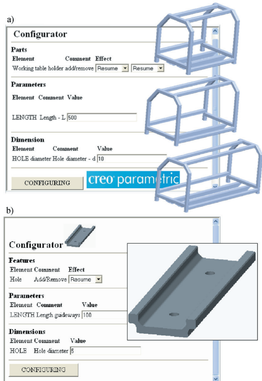
Fig. 9. CAD configurators in Pro/WEB.Link a) supporting structure b) Igus guideways
