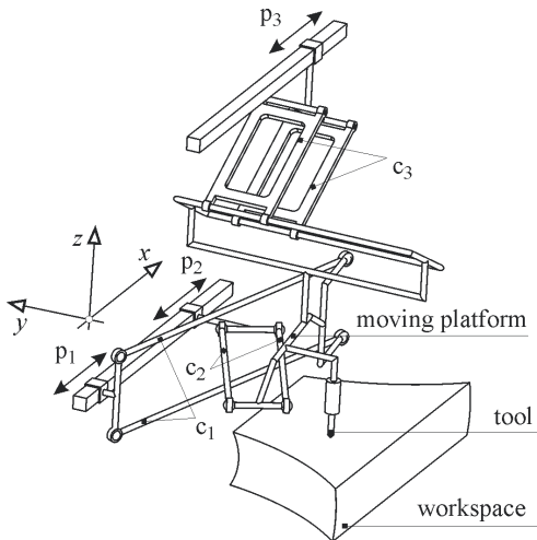
Fig. 4. Parallel mechanism pn101 [13]
