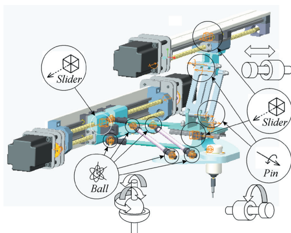
Fig. 12. CAD model for the simulation of mechanism kinematics
