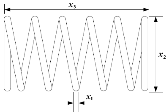
Figure 4: Tension/Compression Spring.
