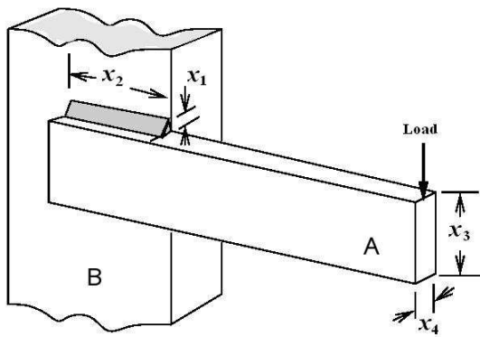
Figure 1: Weldem Beam.
