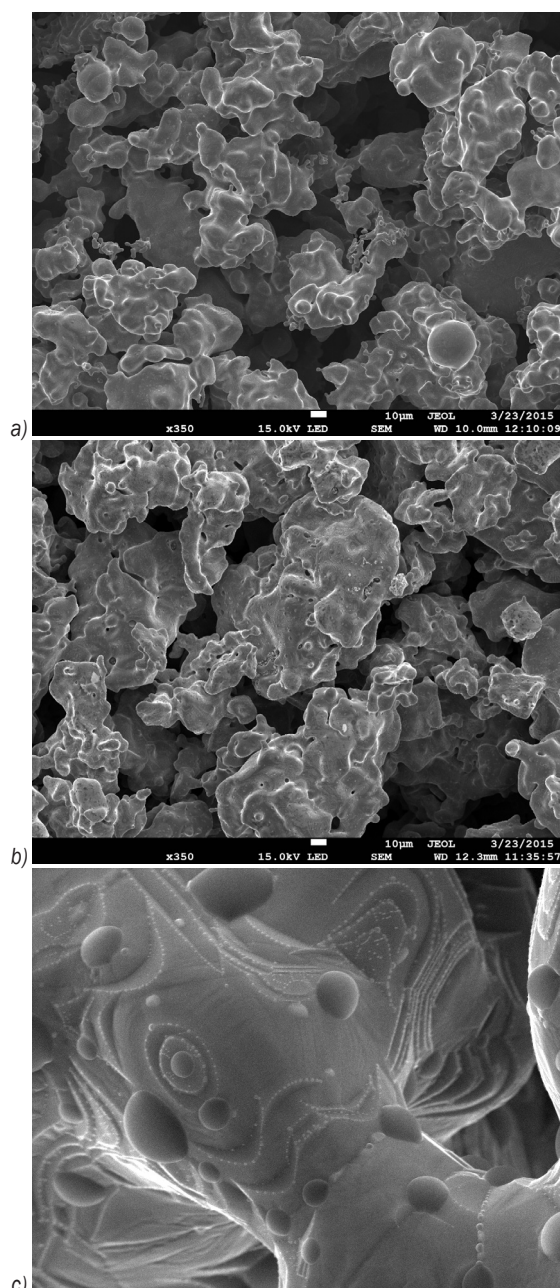
Fig. 2. SEM images of the sintered iron based powders: a) ASC (magnification 350x), b) SE (magnification 350x) and c) SE (magnification 5000x), a bridge between particles visible
