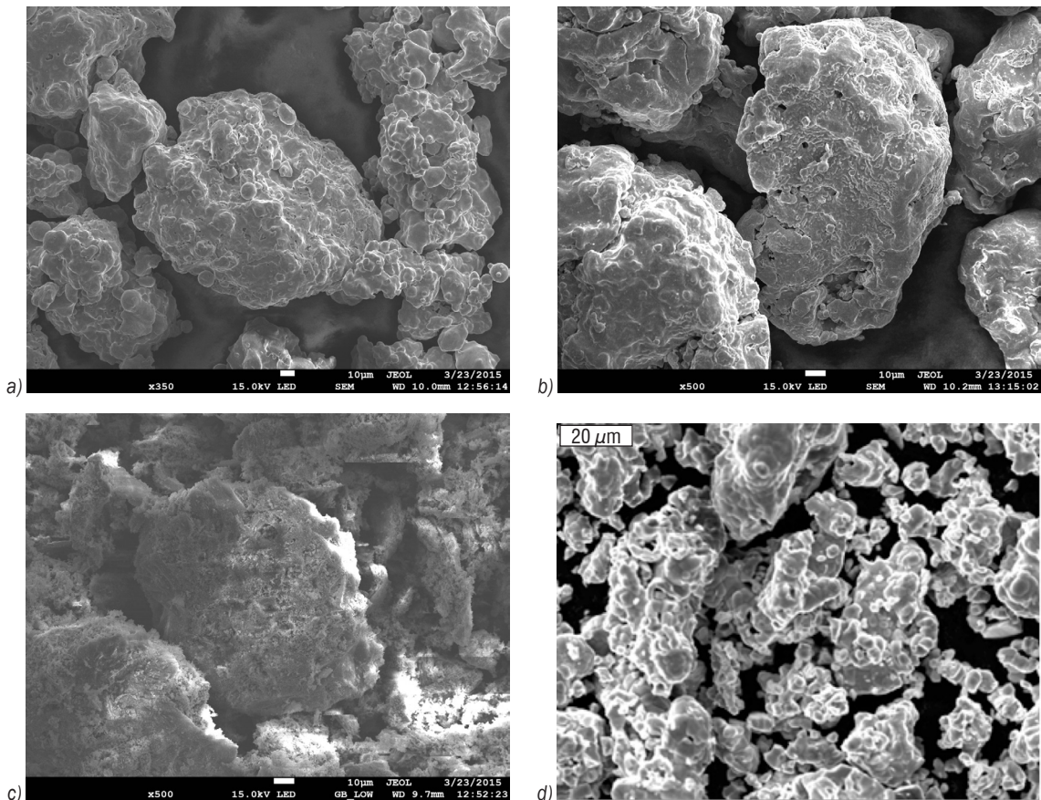
Fig. 1. SEM images of the constituent powders: a) ASC 100.29, b) DISTALOY SE, c) iron (III) oxide, and d) copper
