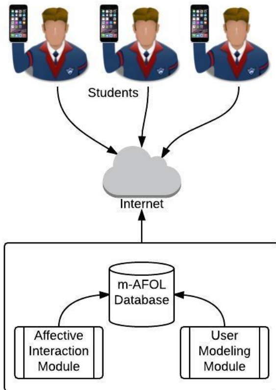
Figure 1: m-AFOL Architecture.
