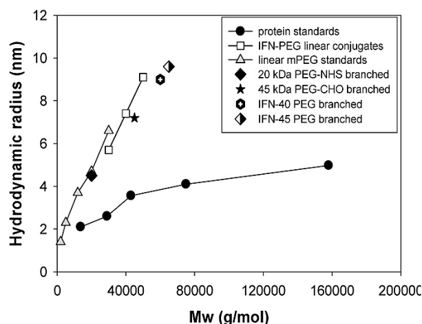
Figure 4: DLS measurements of hydrodynamic radius of linear mPEG standards, branched PEG reagents, protein standards and PEG-IFN conjugates.
