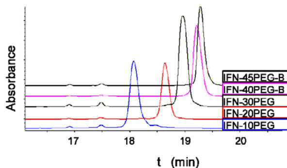
Figure 7: Reversed phase chromatography of PEG-IFN conjugates: IFN-10PEG, IFN-20PEG, IFN-30PEG, IFN-40PEG branched, IFN-45PEG branched.
