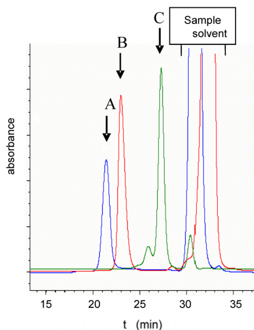
Figure 1: SEC analysis of mPEG-CHO reagent derivatized with pAB (40 kDa) (A – blue), IFN-20PEG, (38 kDa) and (B – red) ovalbumin (43 kDa) (C – green) on TSKgel G4000SWxl (Tosoh Bioscience, Japan). Main peaks are marked with arrows.
