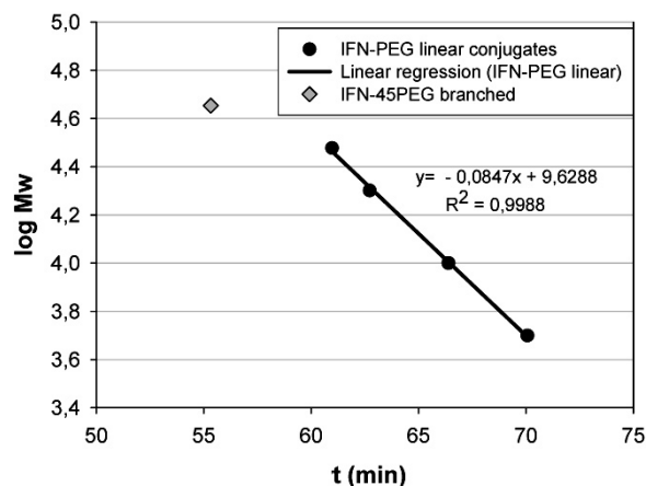
Figure 6: Calibration curves for CEC analysis of N terminally pegylated IFN conjugates shown in Fig 5.
