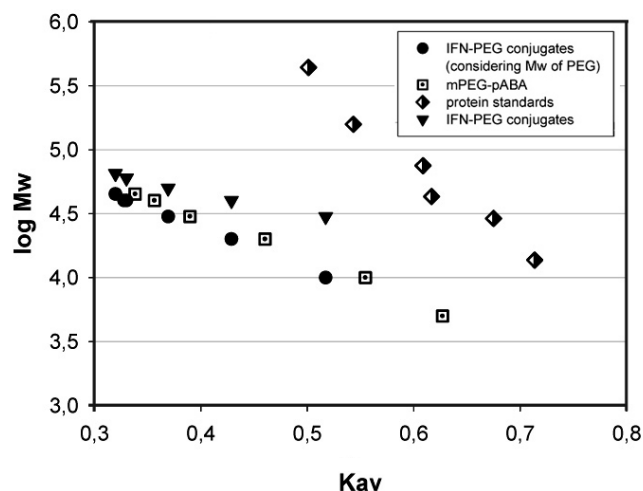
Figure 3: Calibration curves on TSKgel G4000SWxl (Tosoh Bioscience, Japan) for PEG-IFN conjugates (IFN-10PEG, IFN-20PEG, IFN-30PEG, IFN-40PEG branched, IFN-45PEG branched), mPEG-pABZ (5, 10, 20, 30, 40 kDa and branched 45 kDa) and protein standards (Amersham Biosciences) of molecular mass: 13,7, 29, 43, 75, 158 and 440 kDa.
