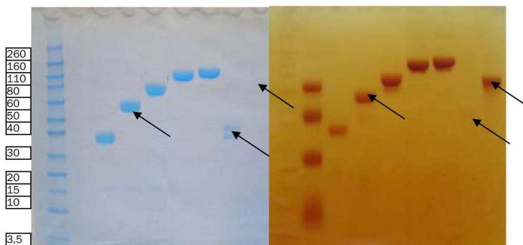
Figure 2: SDS-PAGE of mPEG-OH standards, PEG-IFN conjugates and ovalbumin – Simply Blue Safe stained (a), iodine stained (b)
