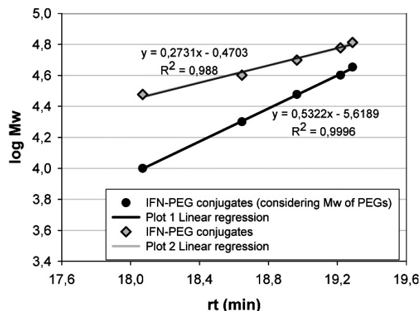
Figure 8: Calibration curves for RP-HPLC analysis of PEG-IFN conjugates shown in Fig 7.
