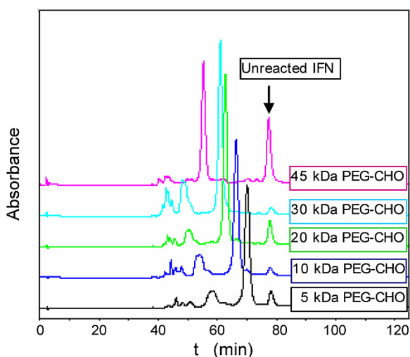
Figure 5: Chromatograms of pegylation mixtures of IFN with various mPEG-CHO reagents of different lengths and shapes (5 kDa linear, 10 kDa linear, 20 kDa linear, 30 kDa linear and 45 kDa branched) on TSK-gel SP-5PW column (Tosoh Bioscience, Japan).
