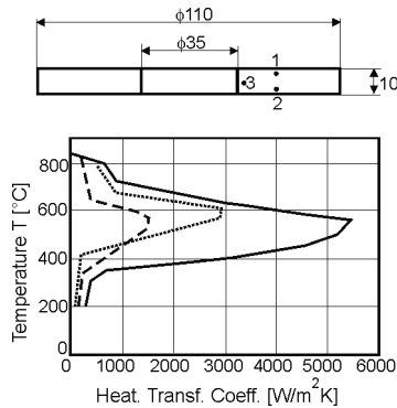
Fig. 5. HTC at different points of a flat ring quenched horizontally in still oil of 70°C [4]
