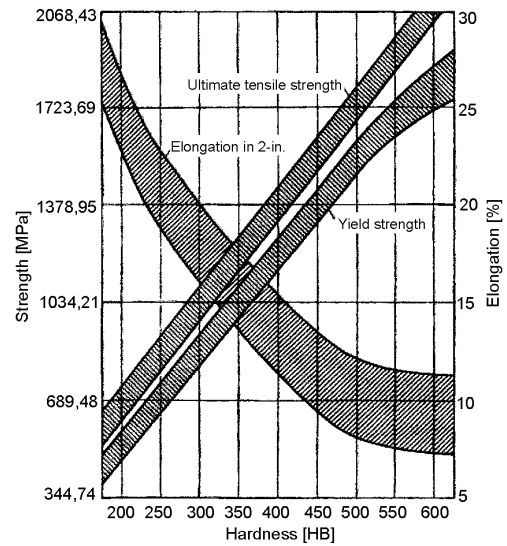
Fig. 20. Range of tensile properties in several quenched and tempered steels at the relevant hardness values [14]
